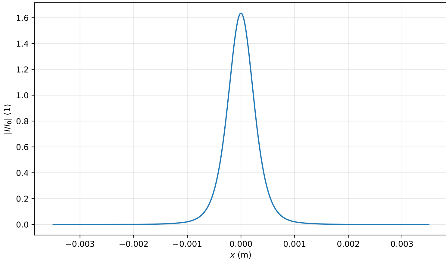
Intensity profile I(x, y = 0, z = 2.149m)/I_0 , P_{in}=0.9P_{cr} , artificial time
